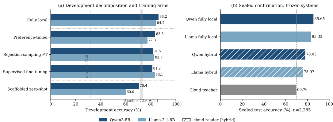
Figure 2: Home-benchmark results. Colours denote the base model in both panels, and hatching marks systems that read questions with the cloud model. (a) Development decomposition. The scaffolded zero-shot rung is the untrained baseline, the three training arms branch from the supervised model, and the fully local rung replaces the cloud reader with a trained local one on top of the best arm per base. The preference-tuned arm shows the base-dependent instability discussed in Section 3.4, and the shaded band covers three cloud-teacher runs. (b) Sealed-test confirmation of the five frozen systems. Intermediate arms never touch the sealed test, which admits one pass per frozen configuration.
