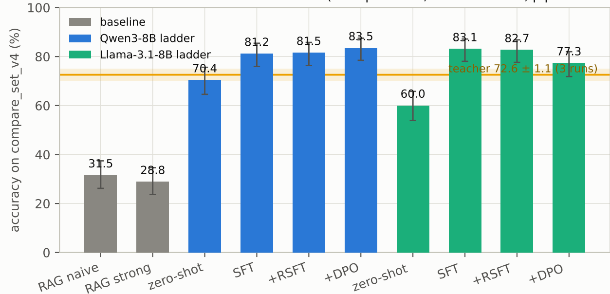
Student ladder vs baselines and teacher (260 questions, Wilson 95% CI, pipeline v2.2)
