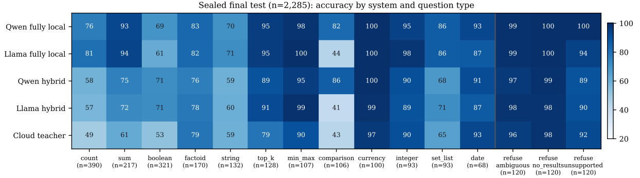
Figure 3: Sealed final-test accuracy by system and question type, twelve answerable types and three refusal classes. The teacher collapses on exhaustive aggregation, comparison skill follows the base model, and the fully local systems close the refusal classes near ceiling.
