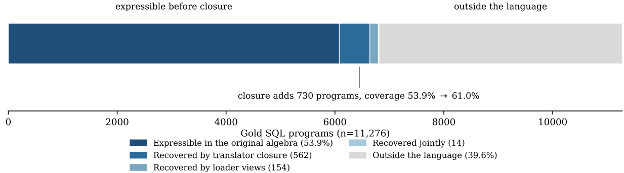
Figure 6: Attribution of WikiTableQuestions program coverage. Compiler and loader closure raise measured coverage from 53.9% to 61.0%, while 39.6% remains outside the language.
