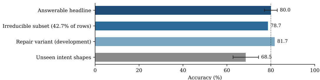
Figure 4: PACS audits. The irreducible subset remains close to the answerable headline, while unseen intent shapes produce the largest measured loss. The repair arm is a development-only variant.
