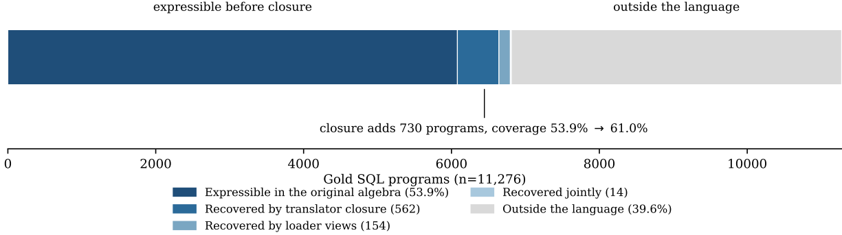
Figure 5: Attribution of WikiTableQuestions program coverage. Compiler and loader closure raise measured coverage from 53.9% to 61.0%, while 39.6% remains outside the language.
