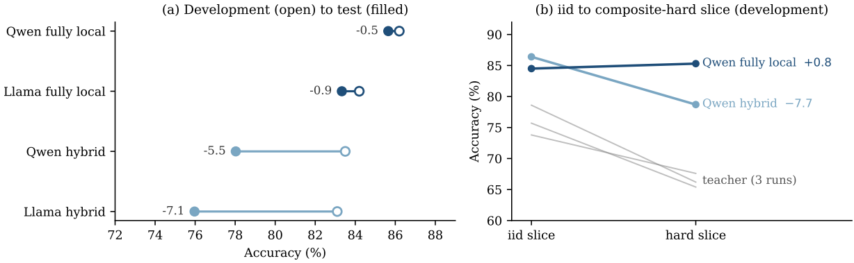
Figure 3: Robustness analyses. (a) Development-to-test movement. (b) IID to composite-hard movement on development data.
