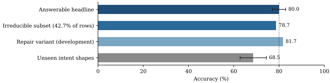
Figure 6: PACS audits. The irreducible subset remains close to the answerable headline, while unseen intent shapes produce the largest measured loss. The repair arm is a development-only variant.
