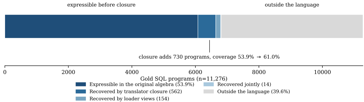
Figure 7: Attribution of WikiTableQuestions program coverage. Compiler and loader closure raise measured coverage from 53.9% to 61.0%, while 39.6% remains outside the language.
