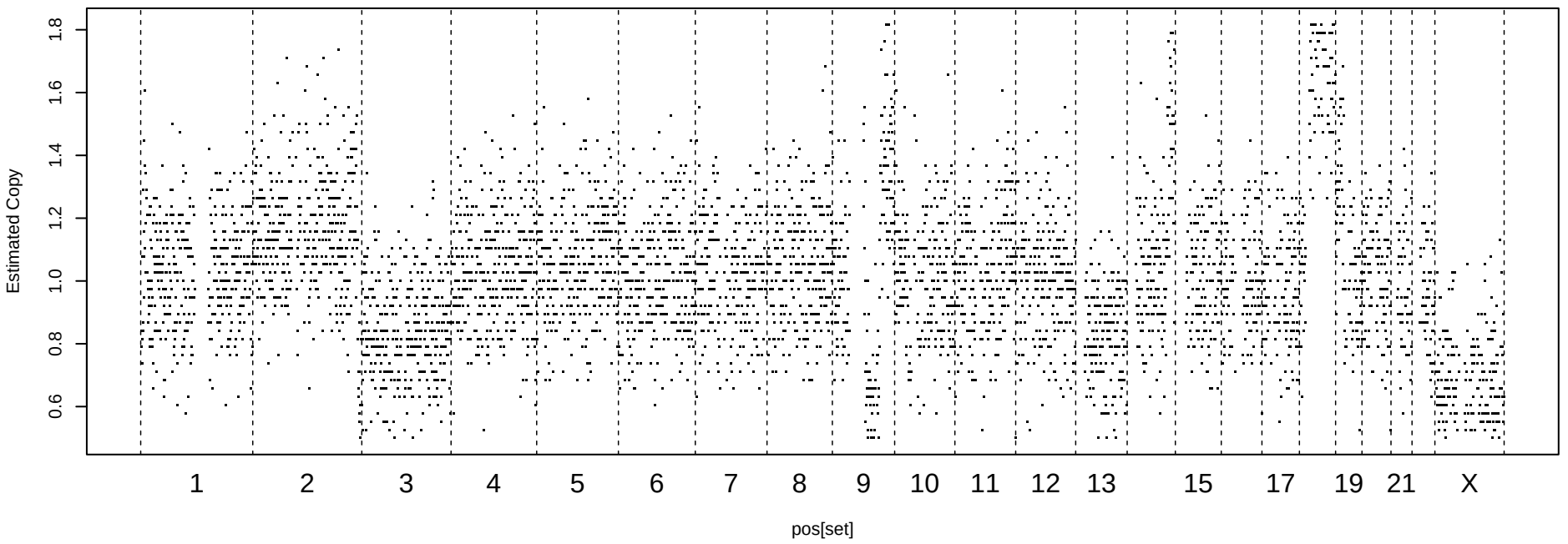
Uncorrected Readcount, MAD = 0.195
