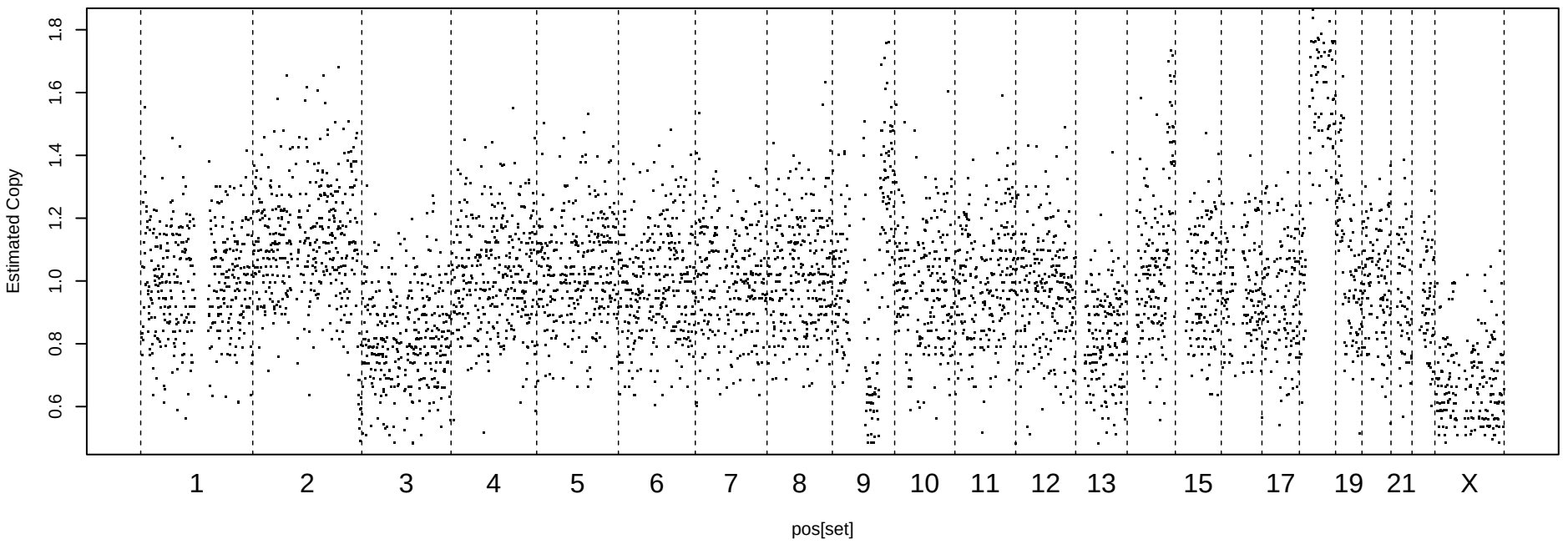
CG-corrected Readcount, MAD = 0.205
