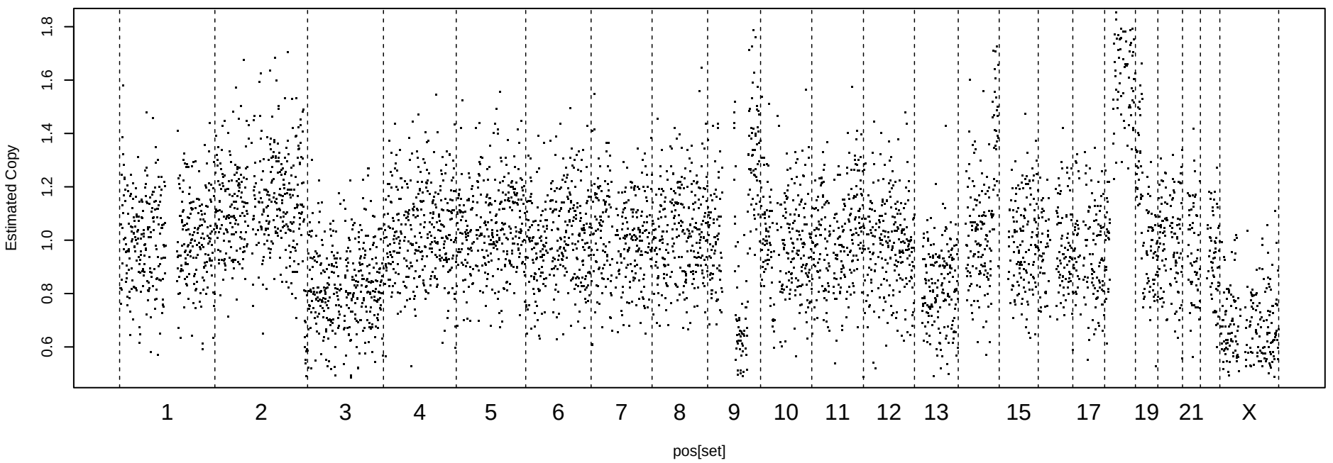
Mappability and GC-corrected Readcount, MAD = 0.207
