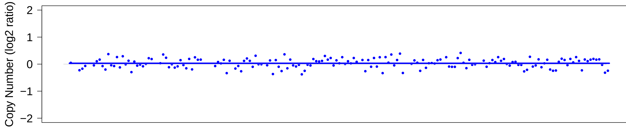
Chromosome chr4
