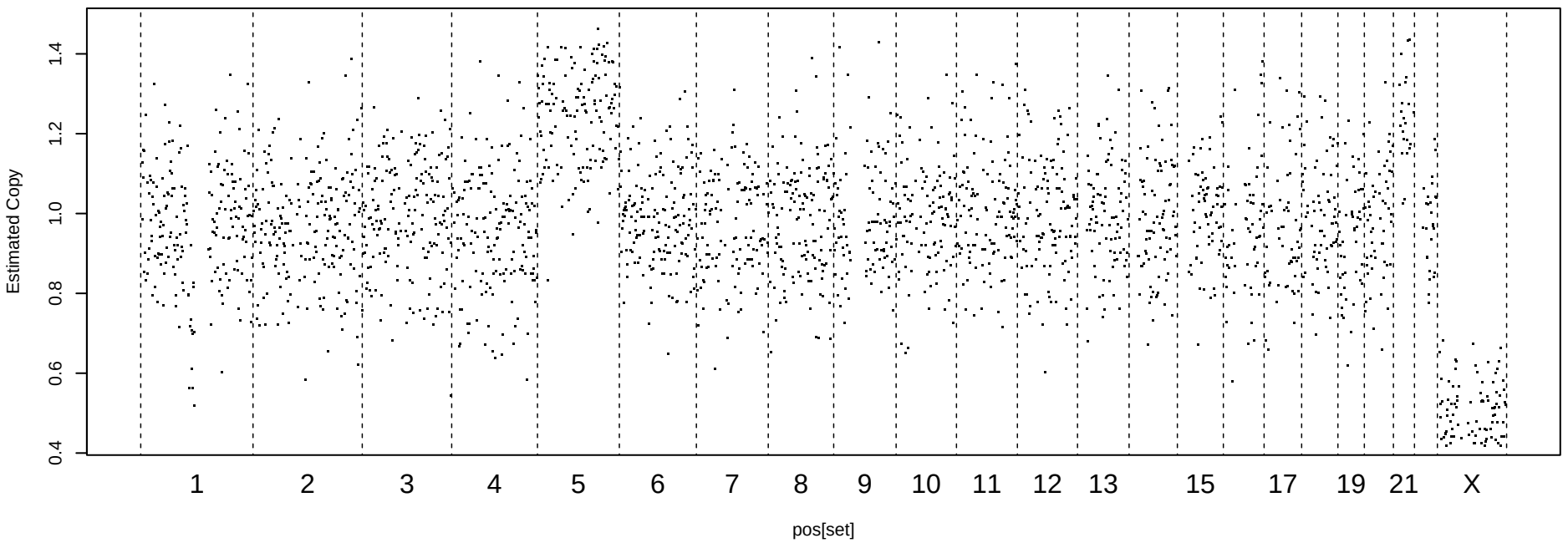
CG-corrected Readcount, MAD = 0.149
