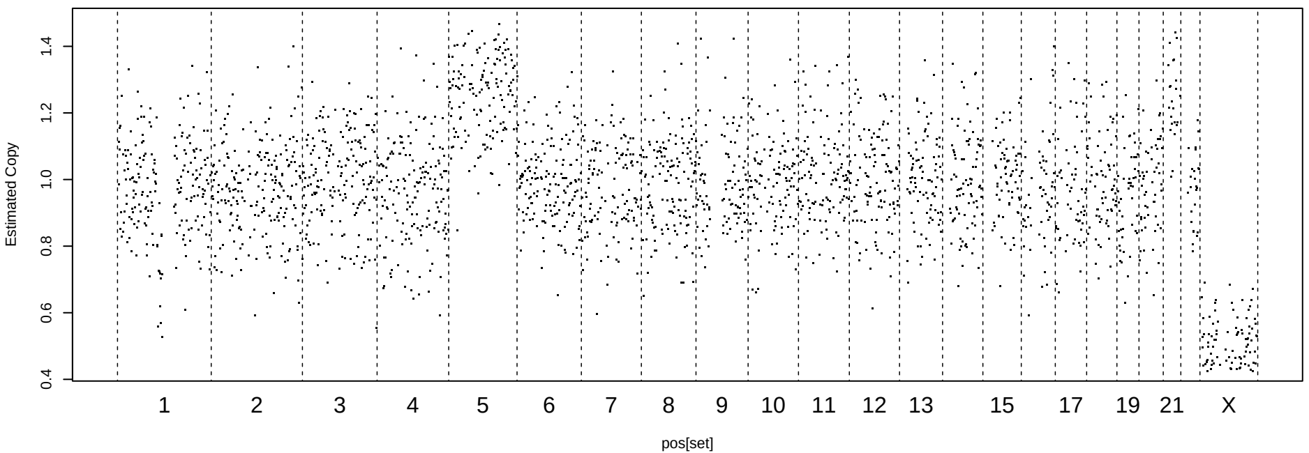
Mappability and GC-corrected Readcount, MAD = 0.152
