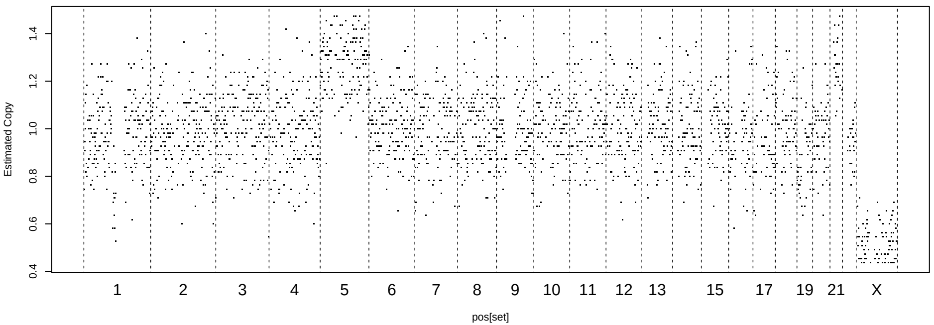
Uncorrected Readcount, MAD = 0.162
