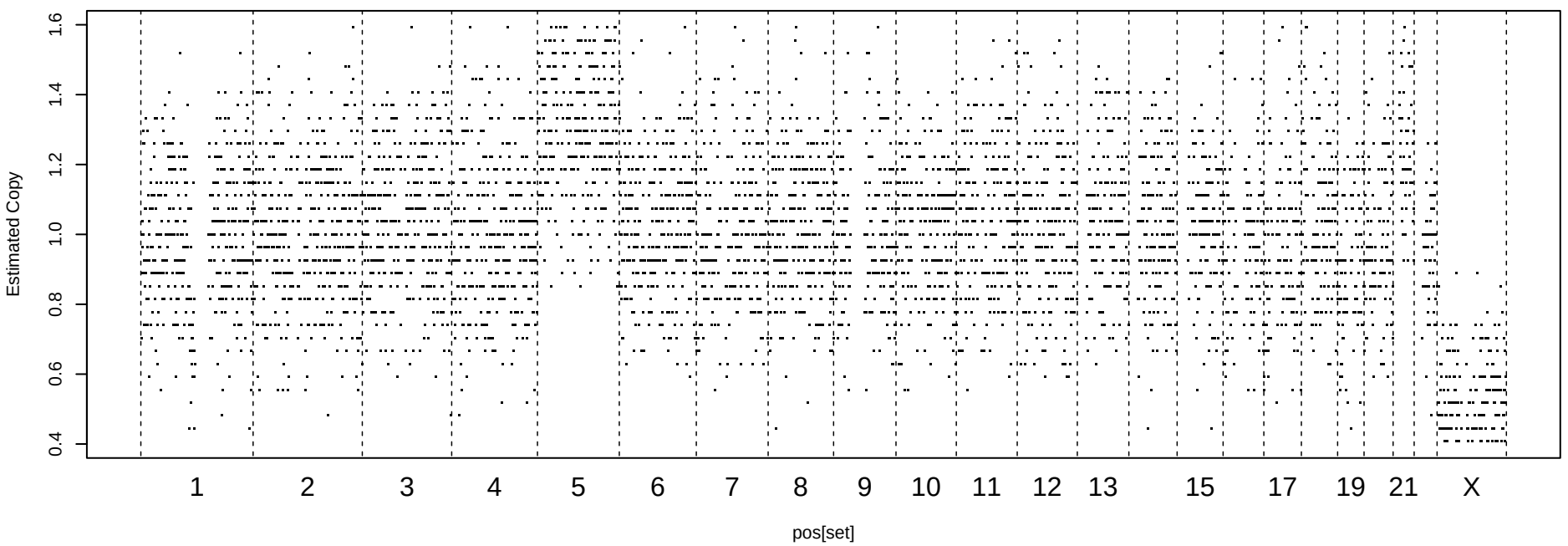
Uncorrected Readcount, MAD = 0.22
