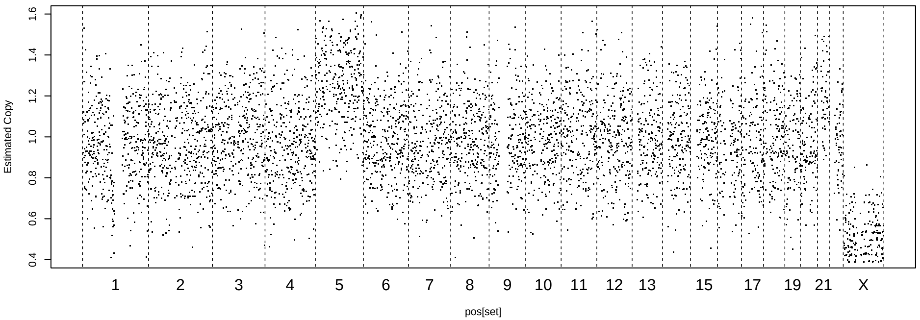
Mappability and GC-corrected Readcount, MAD = 0.21
