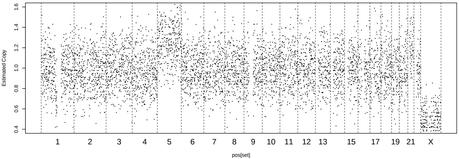
CG-corrected Readcount, MAD = 0.21
