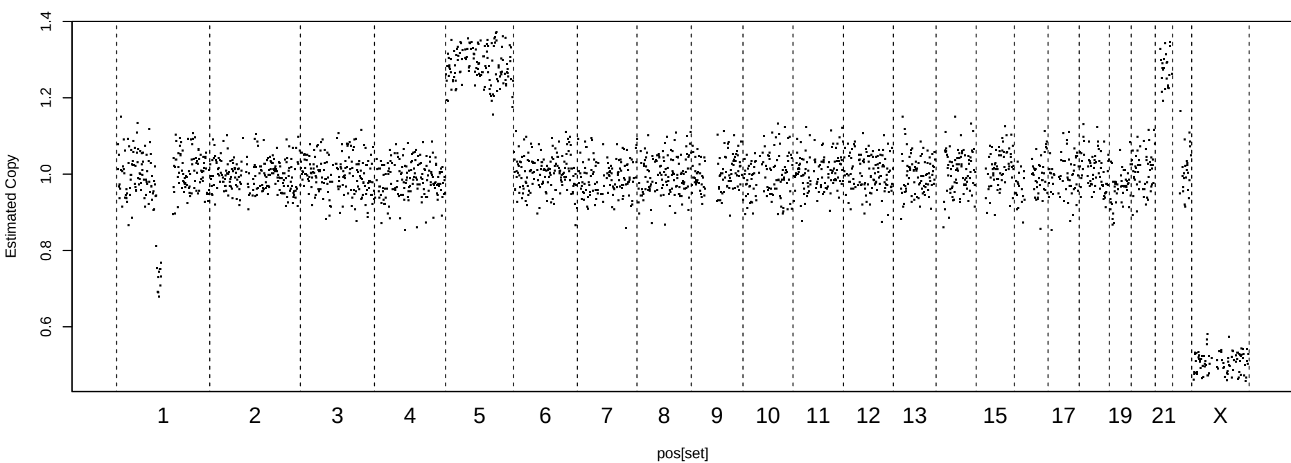
Mappability and GC-corrected Readcount, MAD = 0.0563
