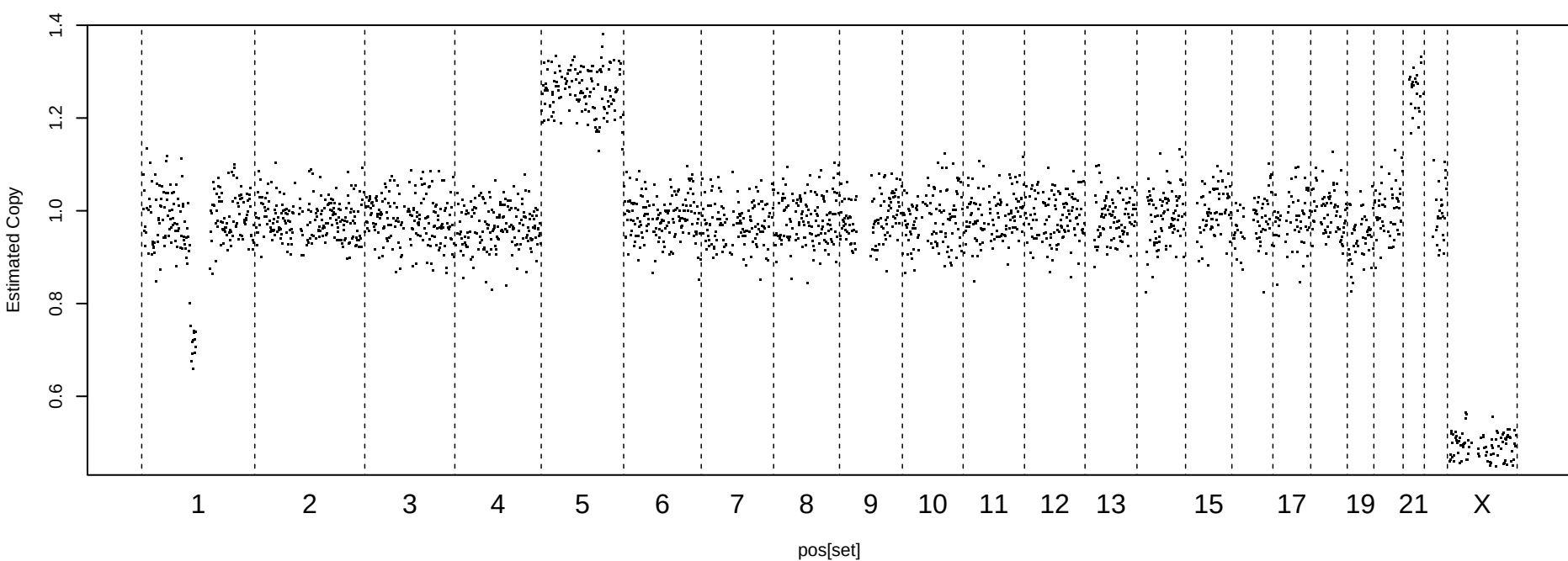
CG-corrected Readcount, MAD = 0.0572
