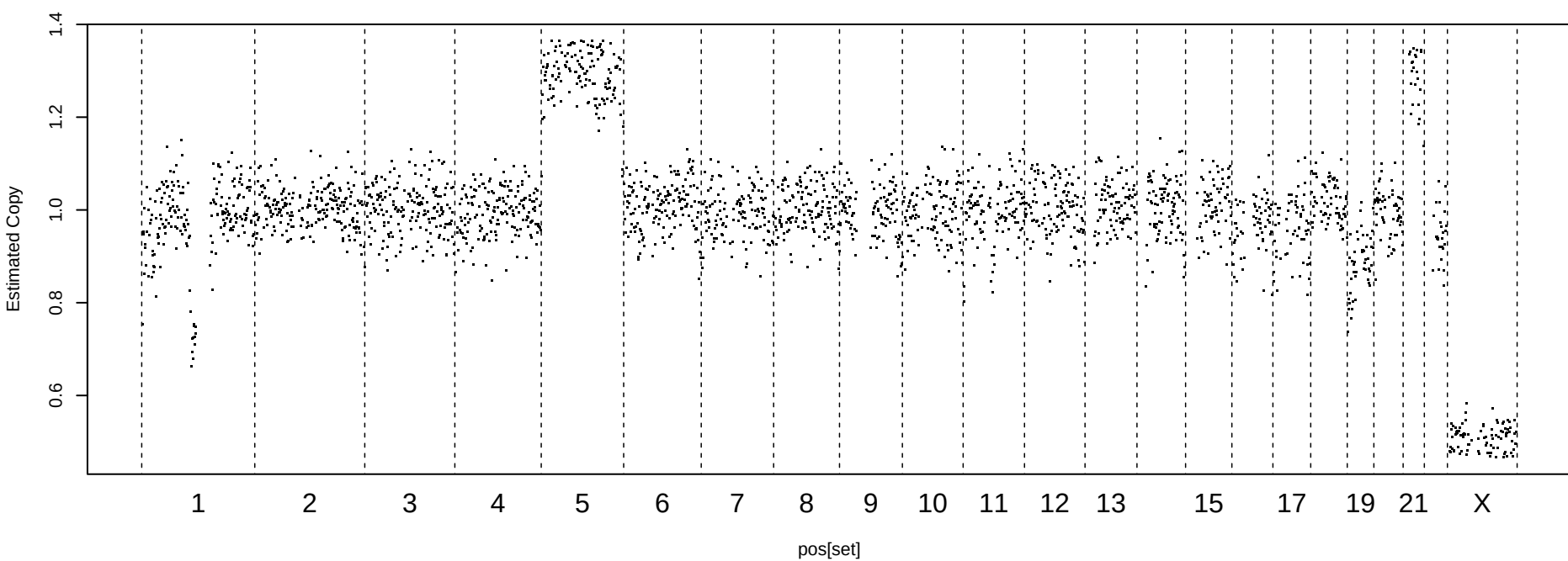
Uncorrected Readcount, MAD = 0.0621
