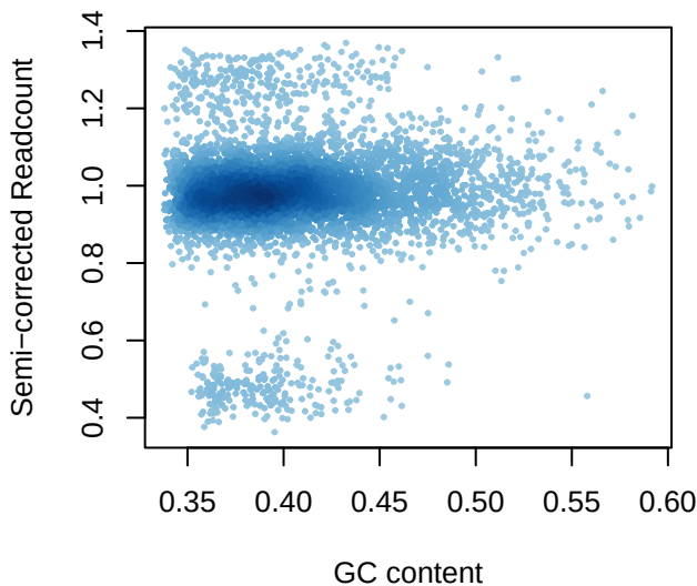
GC Bias in Corrected Readcounts
