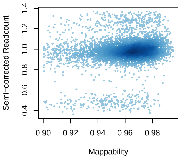
Mappability Bias in GC-Corrected Readcount
