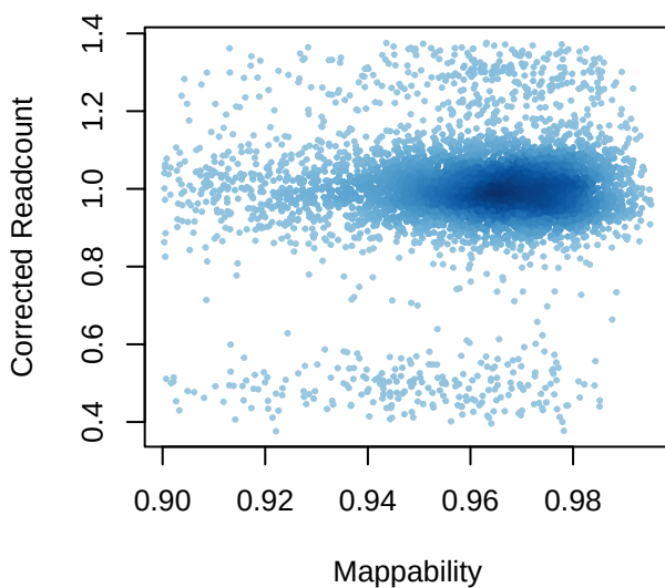
GC and Mappability Corrected Readcount
