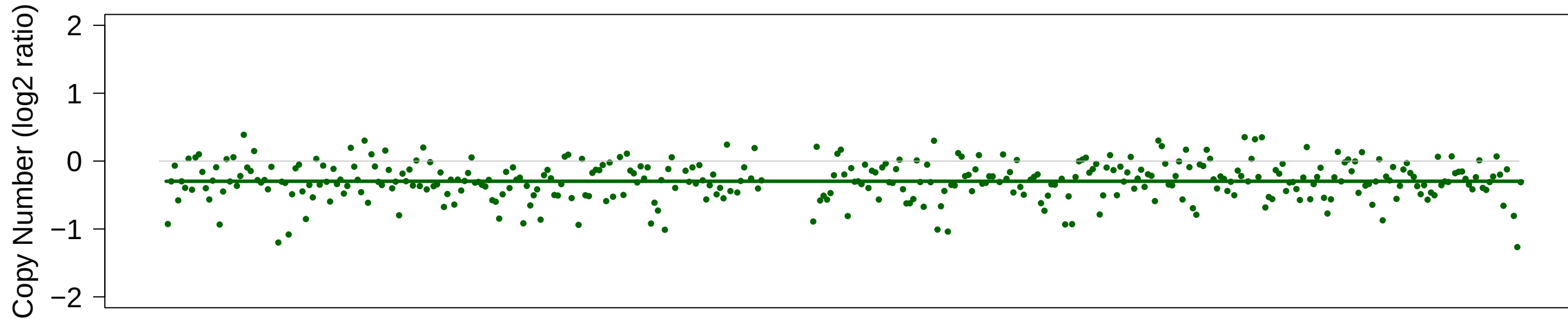
Chromosome chr3
