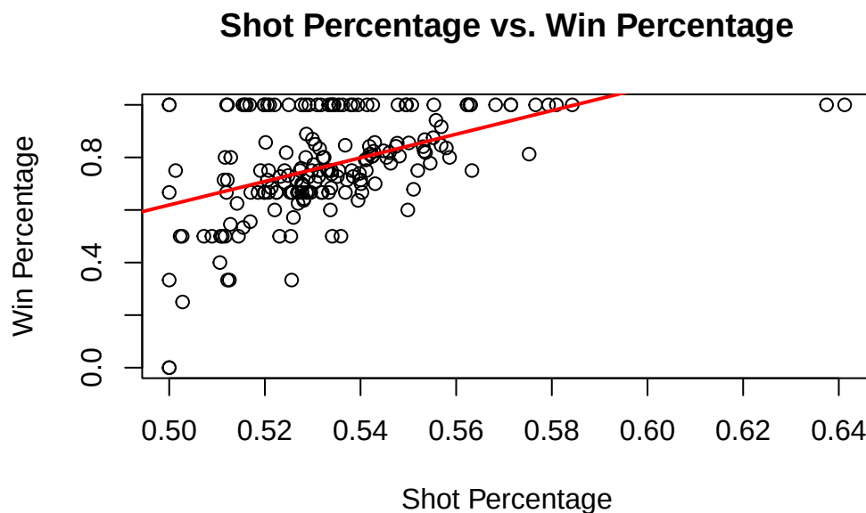
Figure 1: Scatterplot of shot percentage and win percentage with the fitted simple linear regression line.
