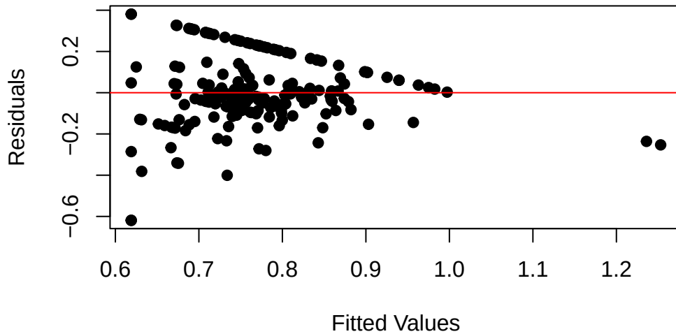
Figure 2: Residuals versus fitted values for the regression model.
