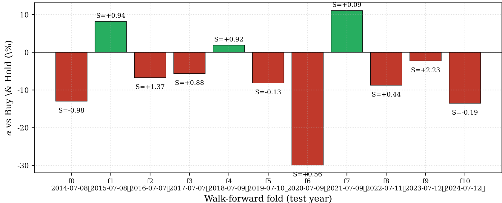
Out-of-Sample Alpha by Year (Walk-Forward 15y, S_1 short)
