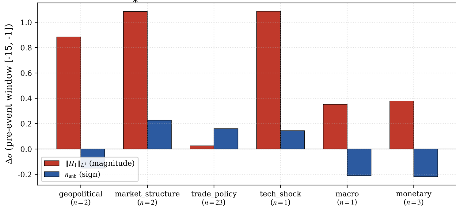
Event Study by Shock Category
