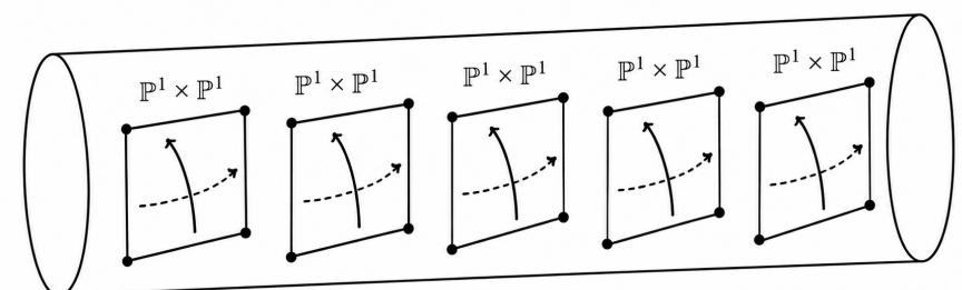
Compactified Jacobian of a two-nodal curve. It is obtained from a \mathbb{P}^1 \times \mathbb{P}^1 -bundle over J(\bar{C}) by two independent translation gluings along the boundary sections.
