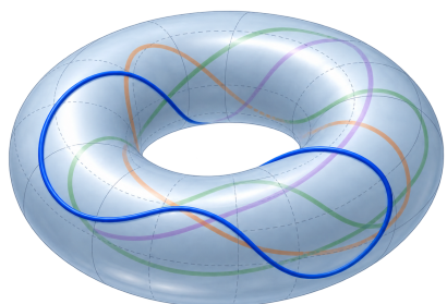
Curves C \in |L| varying on a fixed abelian surface A (schematic).
