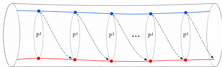
Compactified Jacobian of a one-nodal curve. It is obtained from a \mathbb{P}^1 -bundle over J(\bar{C}) by identifying the two distinguished sections via a translation.
