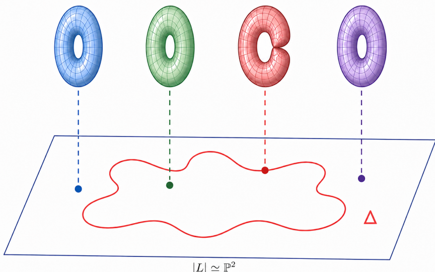
Schematic picture of the relative compactified Jacobian over |L| , with a singular fiber over the discriminant locus \Delta .
