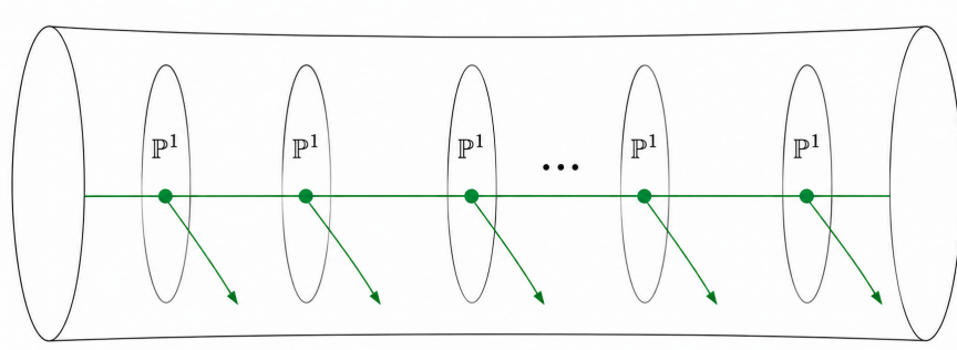
Compactified Jacobian of a cuspidal curve. It is obtained from a \mathbb{P}^1 -bundle over J(\bar{C}) by contracting a distinguished vector field along a section.
