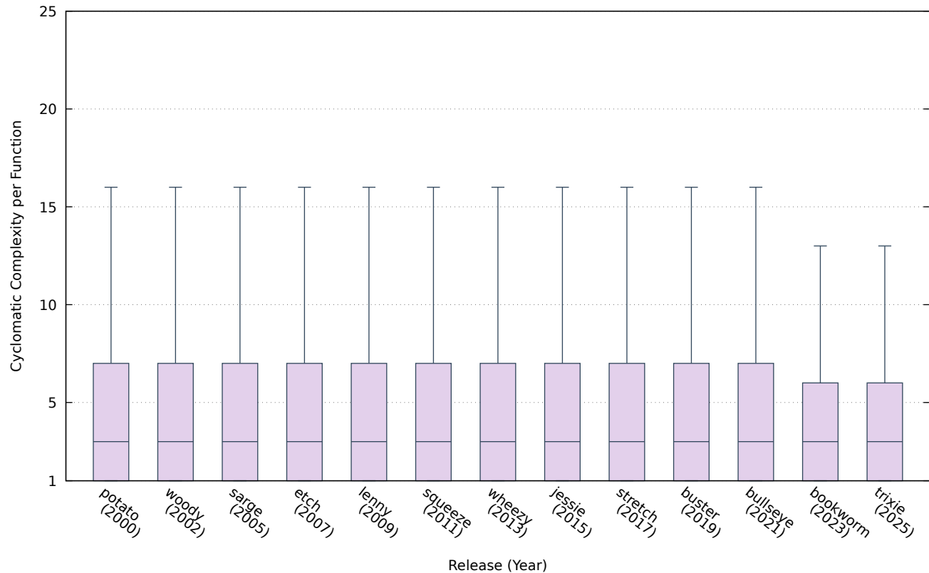
Per-Function Cyclomatic Complexity Distribution per Release
