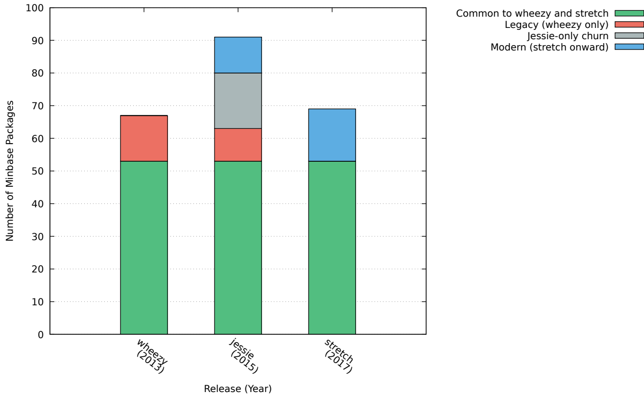
Init-System Transition: Minbase Composition, Wheezy → Jessie → Stretch
