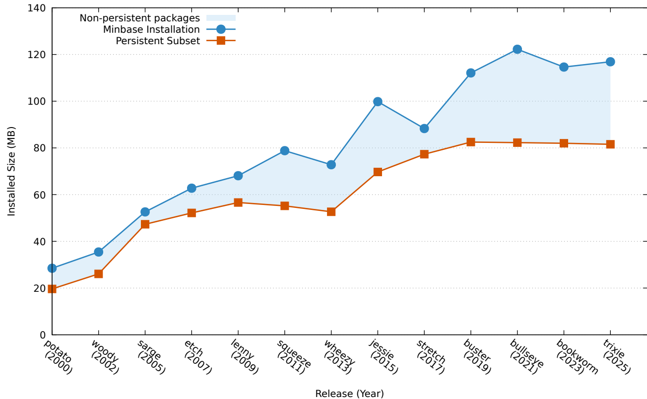
Installed Size of Debian Minbase Installation Over Time
