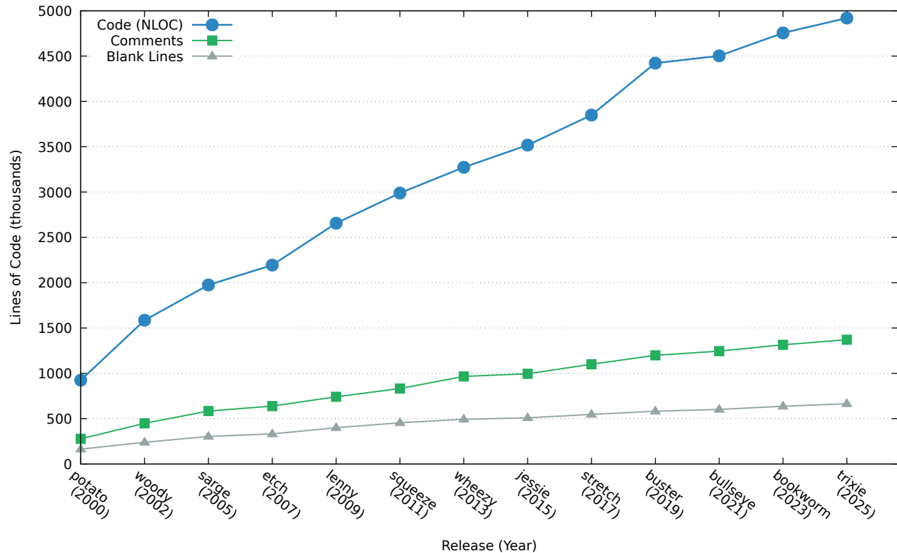
Total Lines of Code in Persistent Base Packages
