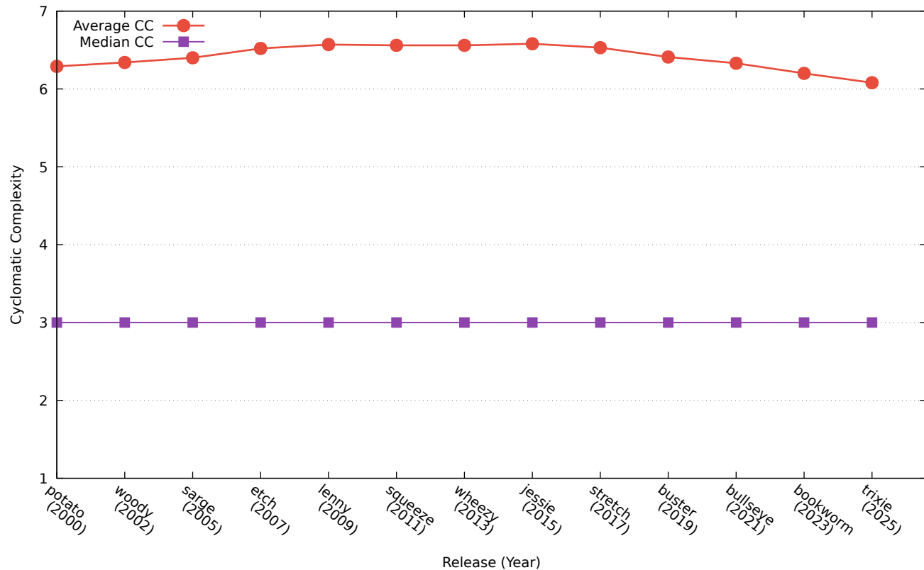
Cyclomatic Complexity of Persistent Base Packages
