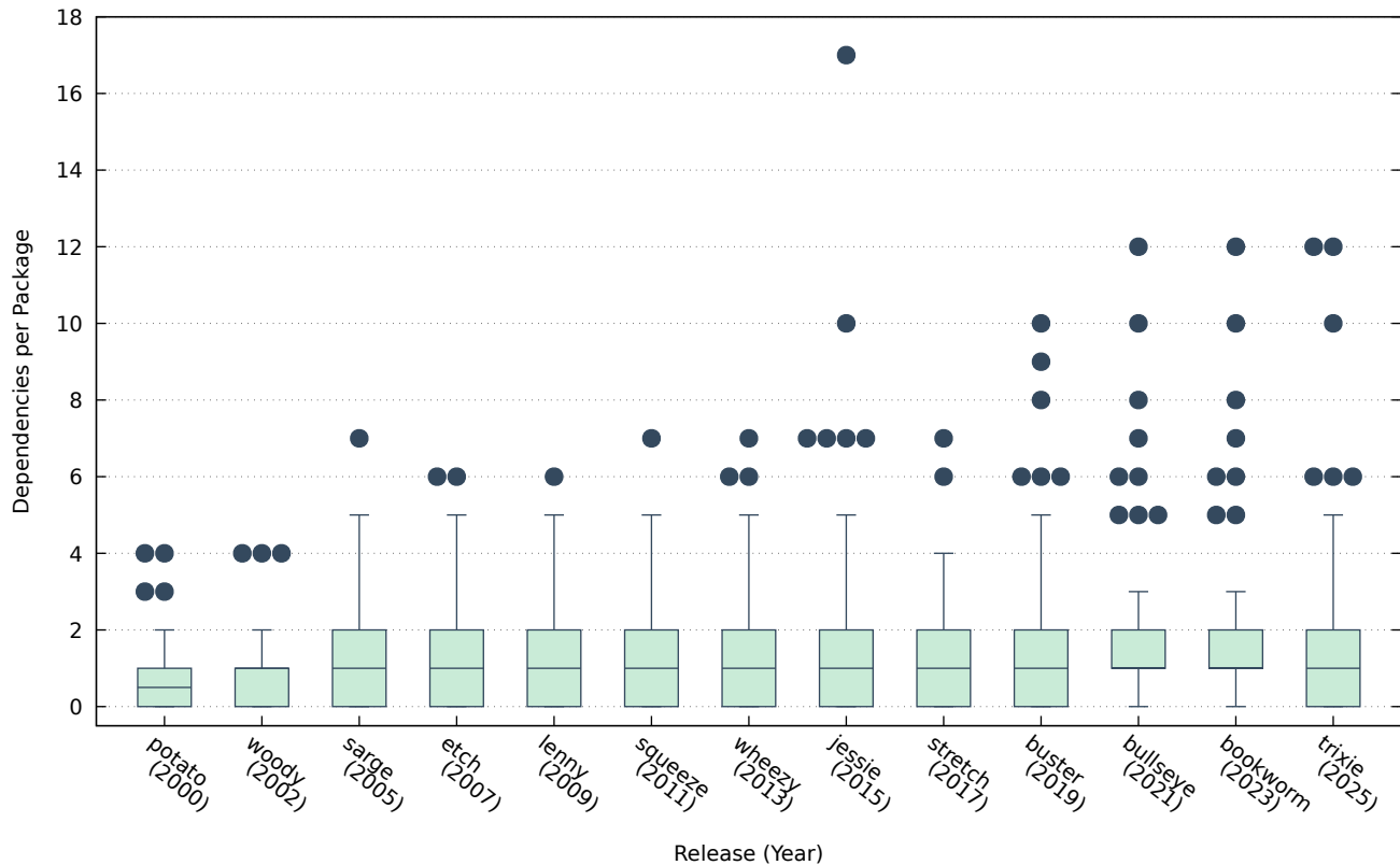
Per-Package Dependency Count Distribution per Release
