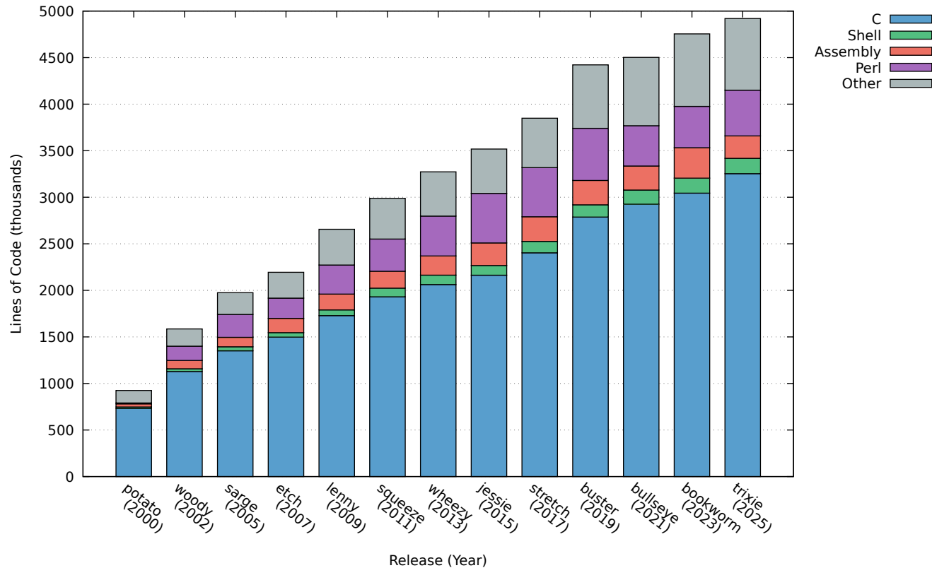
Programming Language Composition in Persistent Base Packages
