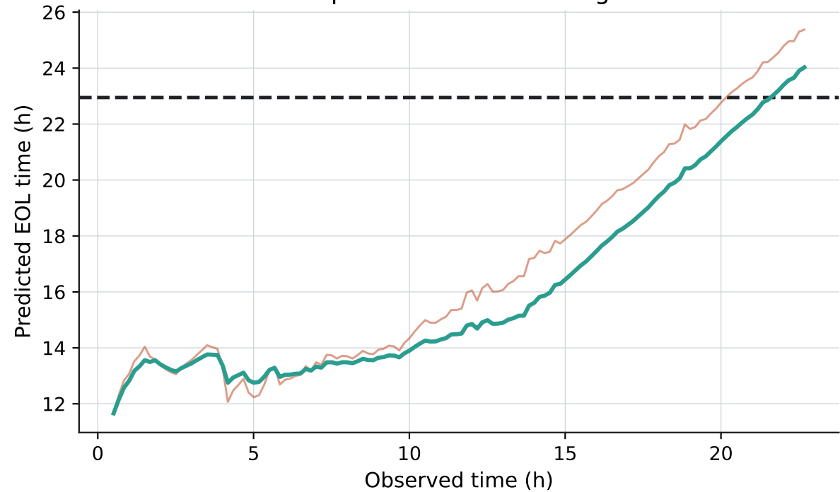
Train4 predicted EOL convergence
