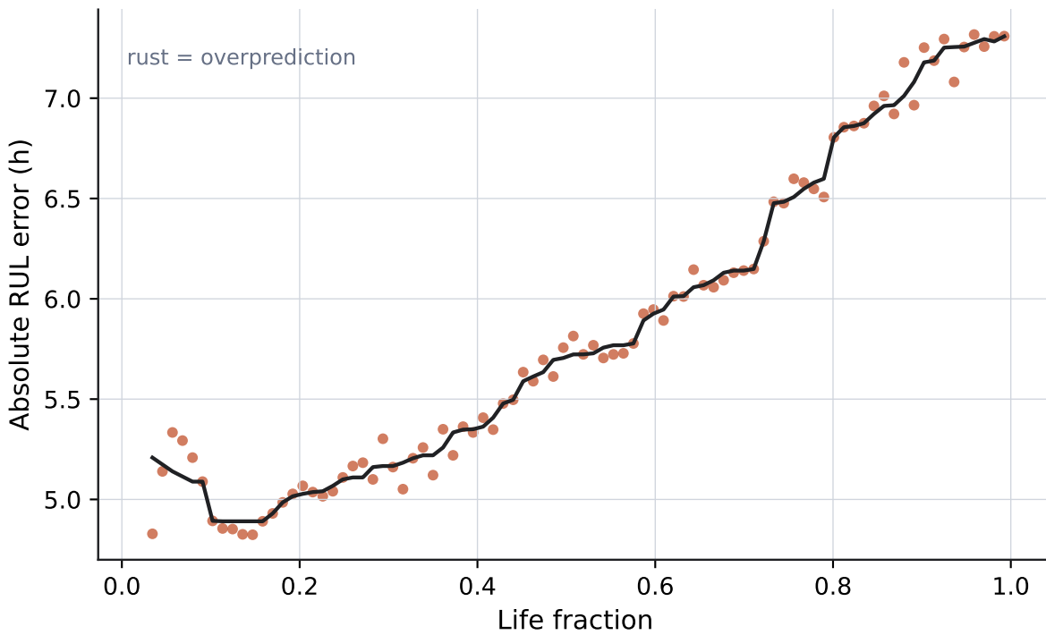
Train3 absolute error over life
