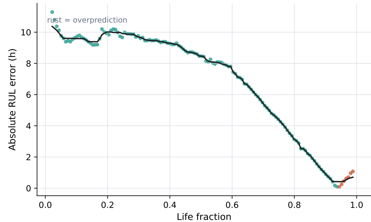
Train4 absolute error over life
