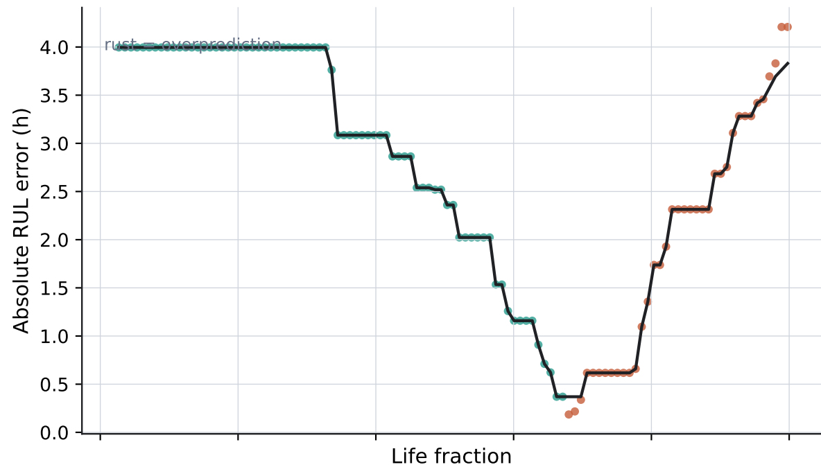
Train4 absolute error over life
