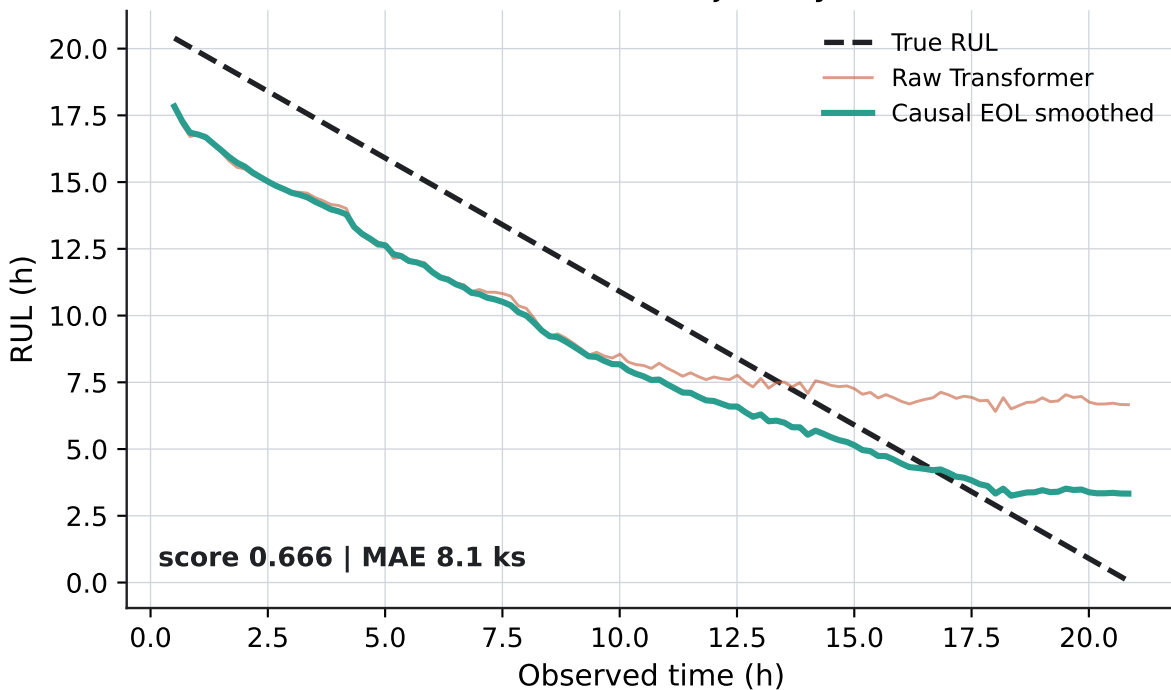
Train3 RUL trajectory
