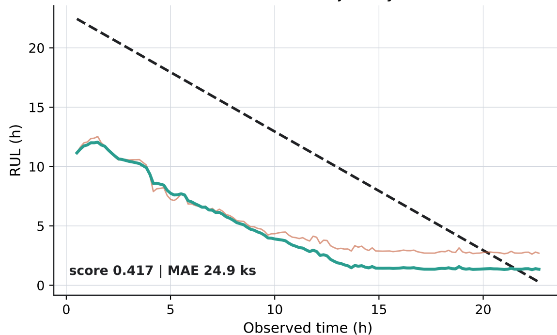
Train4 RUL trajectory
