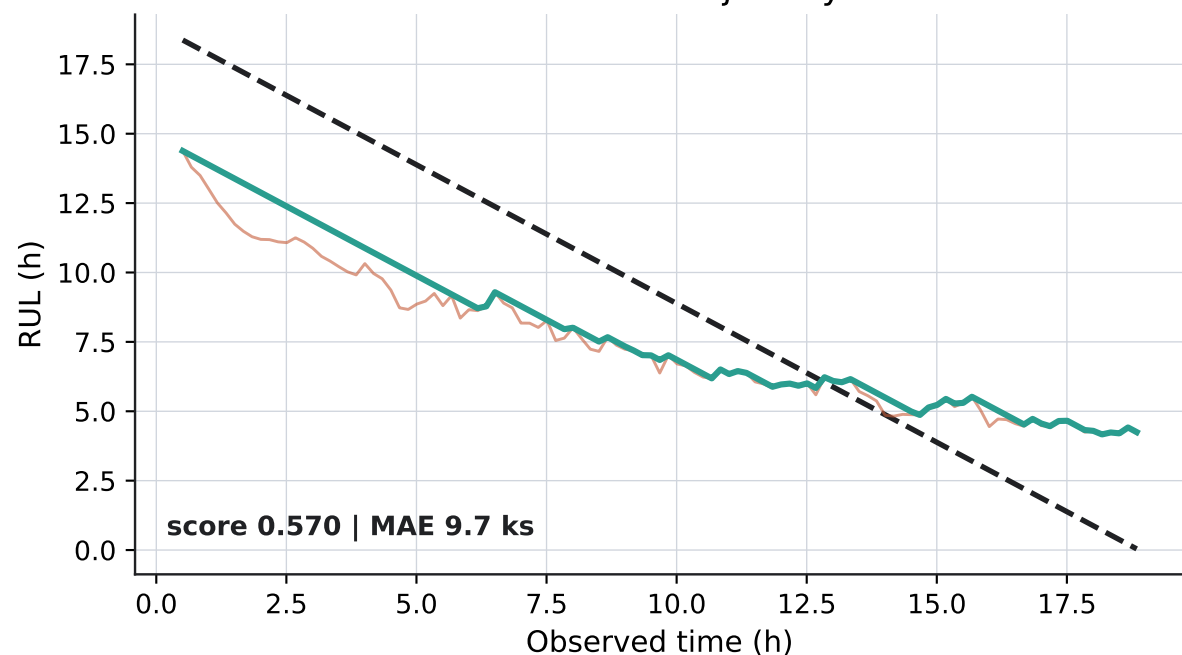
Train4 RUL trajectory
