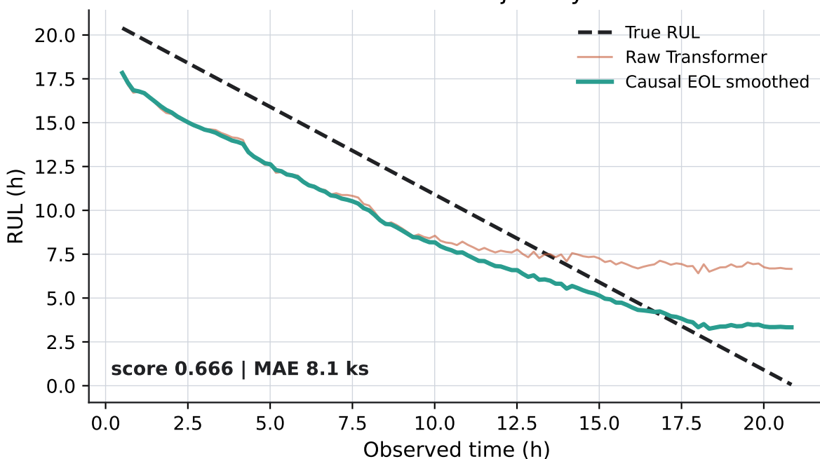
Train3 RUL trajectory
