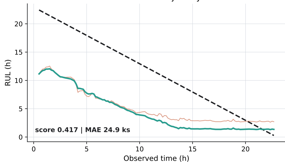
Train4 RUL trajectory
