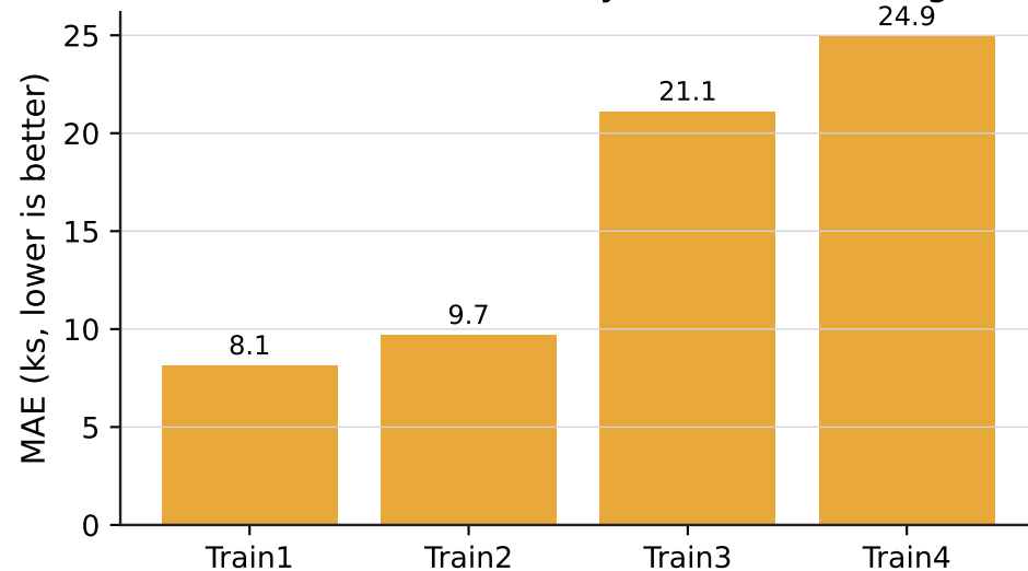
Absolute RUL error by held-out bearing
