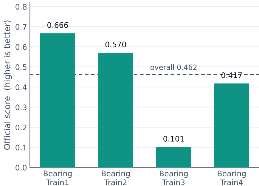
LOBO score by held-out bearing
