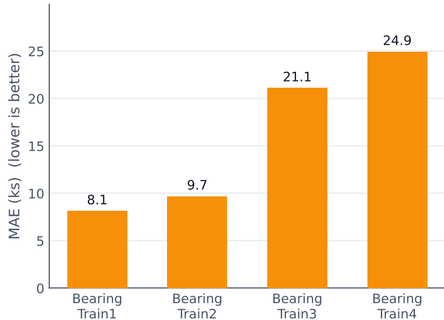
Absolute RUL error by held-out bearing
