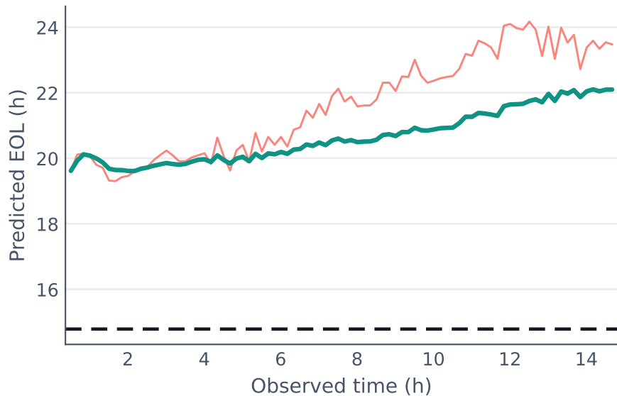
Bearing Train3
