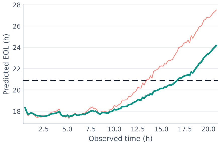
Bearing Train1
