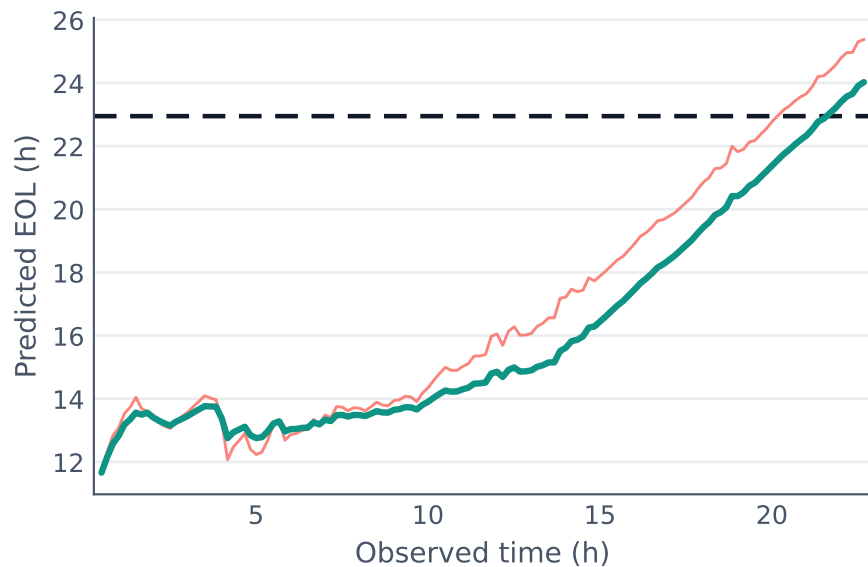
Bearing Train4
