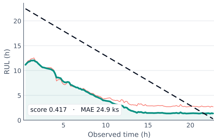
Bearing Train4
