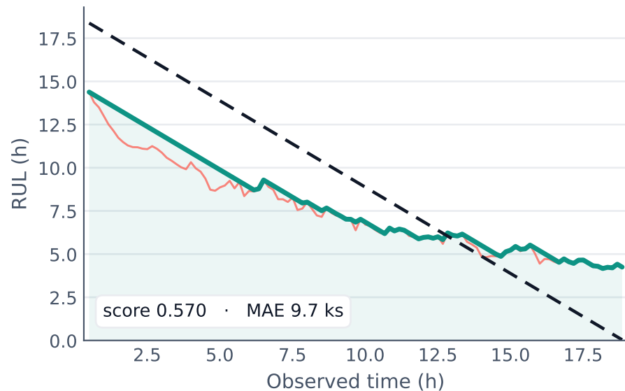
Bearing Train2
