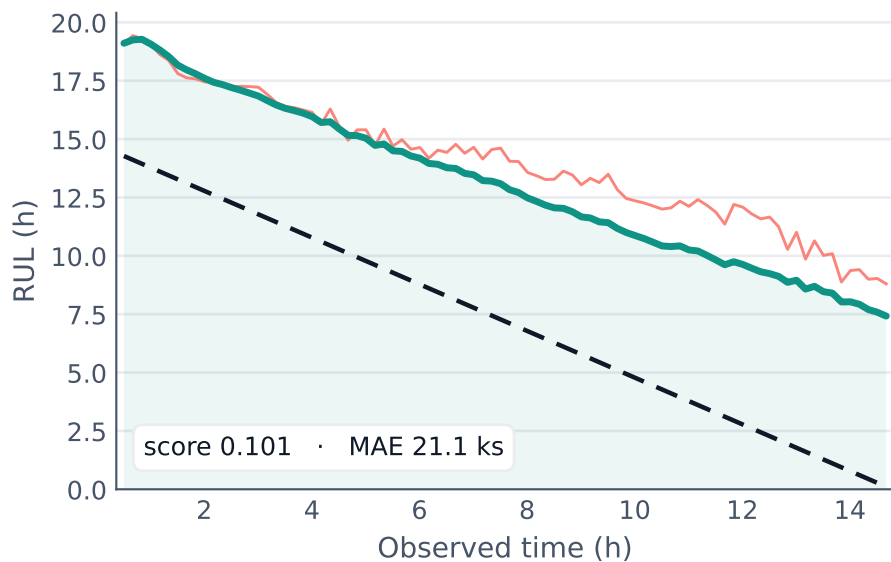
Bearing Train3
