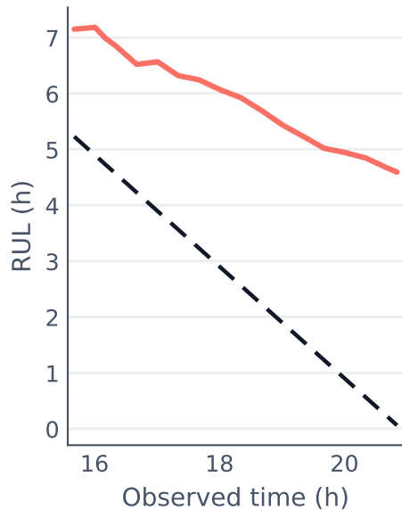
Bearing Train1
