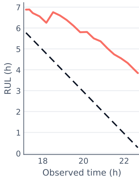
Bearing Train4
