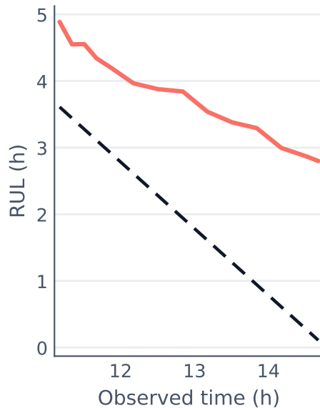
Bearing Train3
