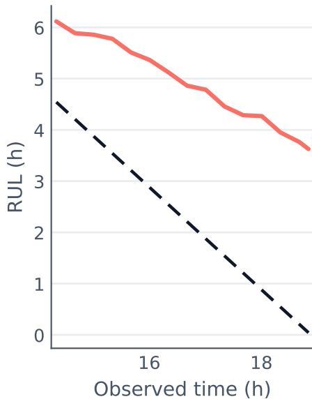
Bearing Train2
