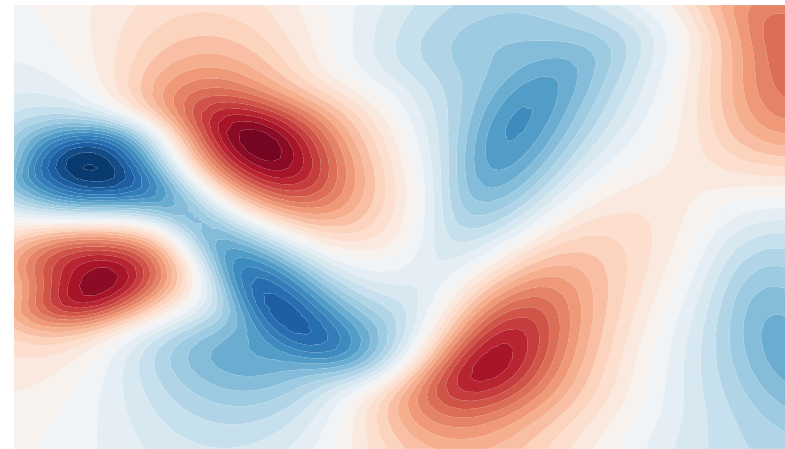
Fluctuation u'
