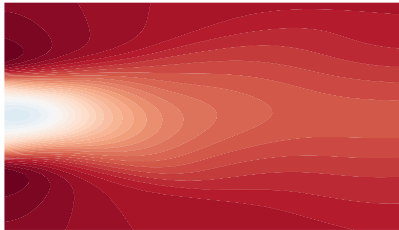
Mean \bar{u}
