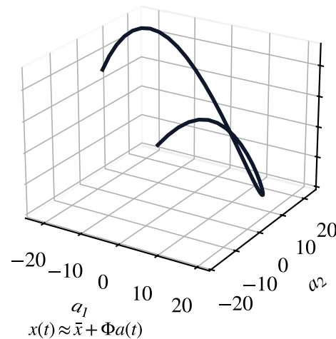
4. Reduced coordinates
