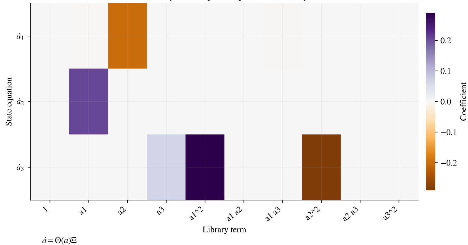
Kutz Cylinder: sparse equation discovery
