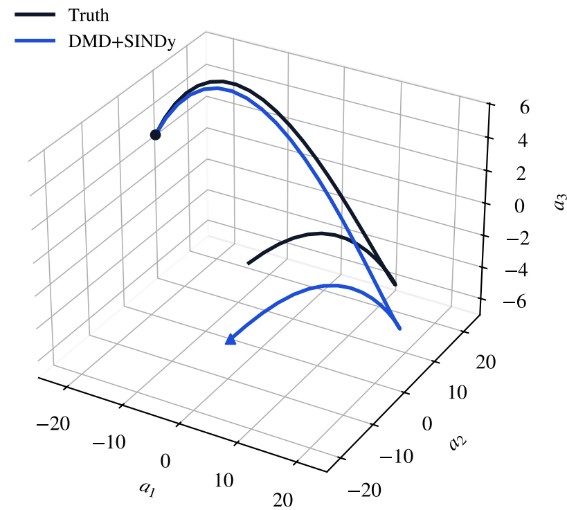
DeepXDE Cylinder (u,v) DMD+SINDy vs Truth (NRMSE=0.088)
