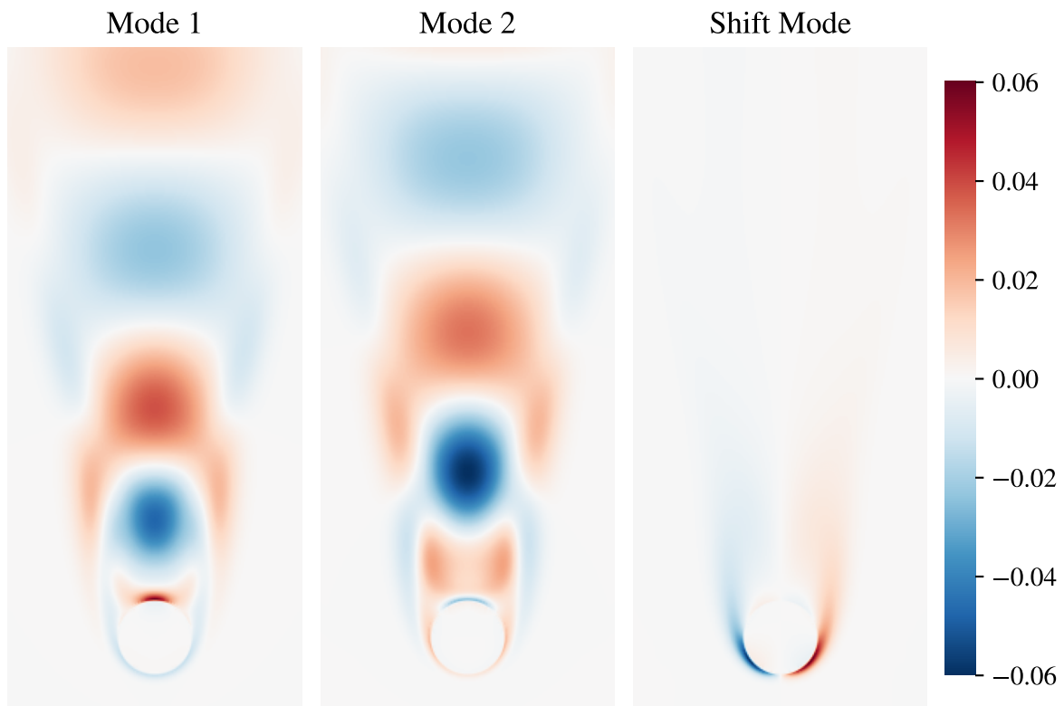
Kutz Cylinder (vorticity)
