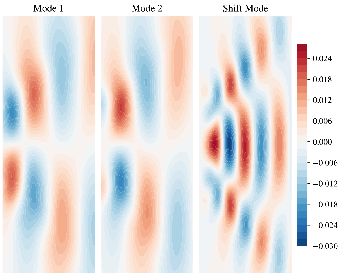
DeepXDE Cylinder (u,v)
