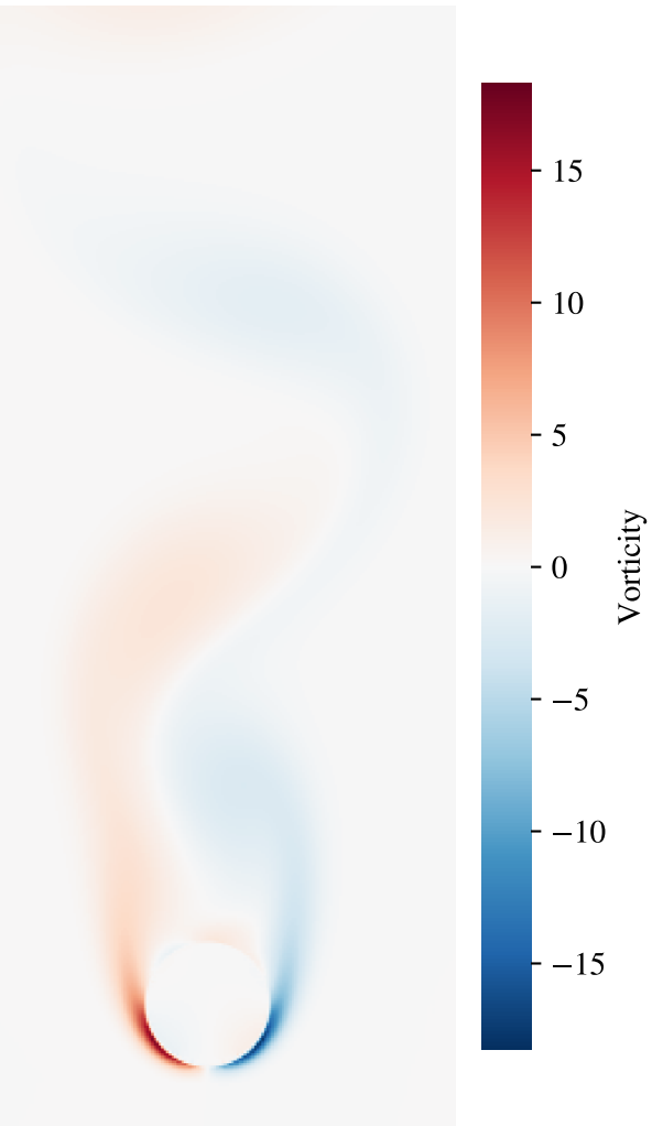
Kutz Cylinder (vorticity) t = 8.00 (5% of record)
