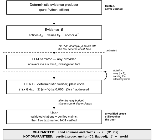
Figure 1: The evidence-bound contract. Tier A binds the tool schema’s enums to E at call time. Tier B re-checks the returned answer in host code, retries with the offending items named, and after the budget strips unsound content and flags a persistent omission. The dashed boundary encloses only the narrator. The producer is trusted and never verified, the free-text field reaches the user marked unverified, and the guarantee is consistency with E , which says nothing about whether E matches the world.
