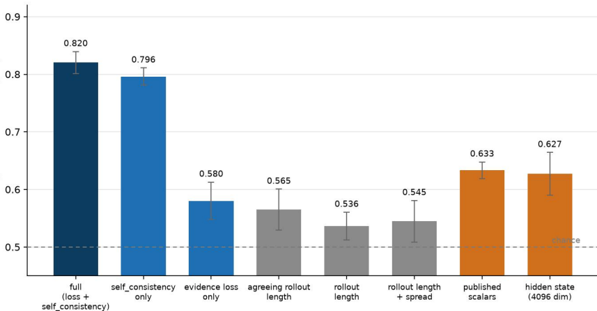
ROC averaged over the five evidence counts main average over four held out groups
