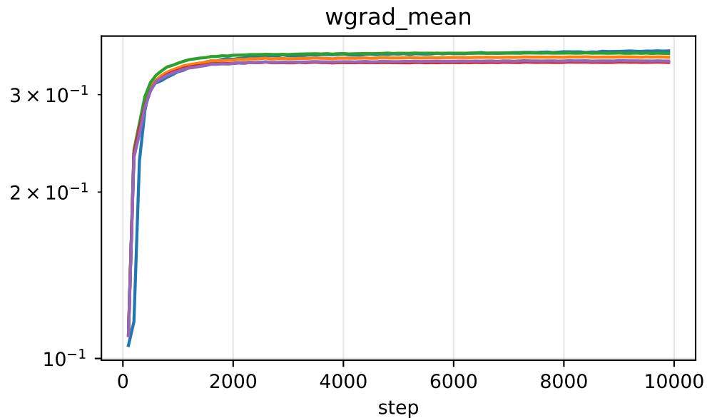
Gradient norms (mean over layers)
