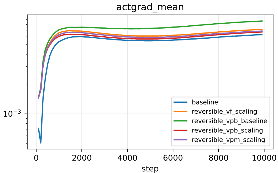
Gradient norms (mean over layers)
