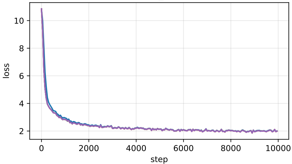
train_loss
