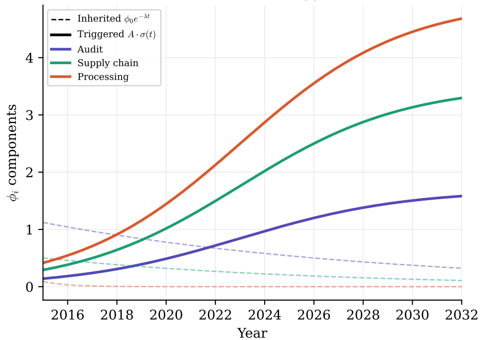
(c) Inherited (dashed) vs. triggered (solid)
