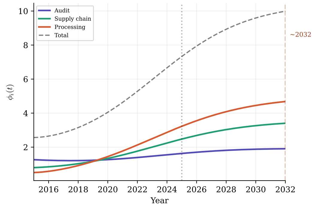
(b) Forward prediction
