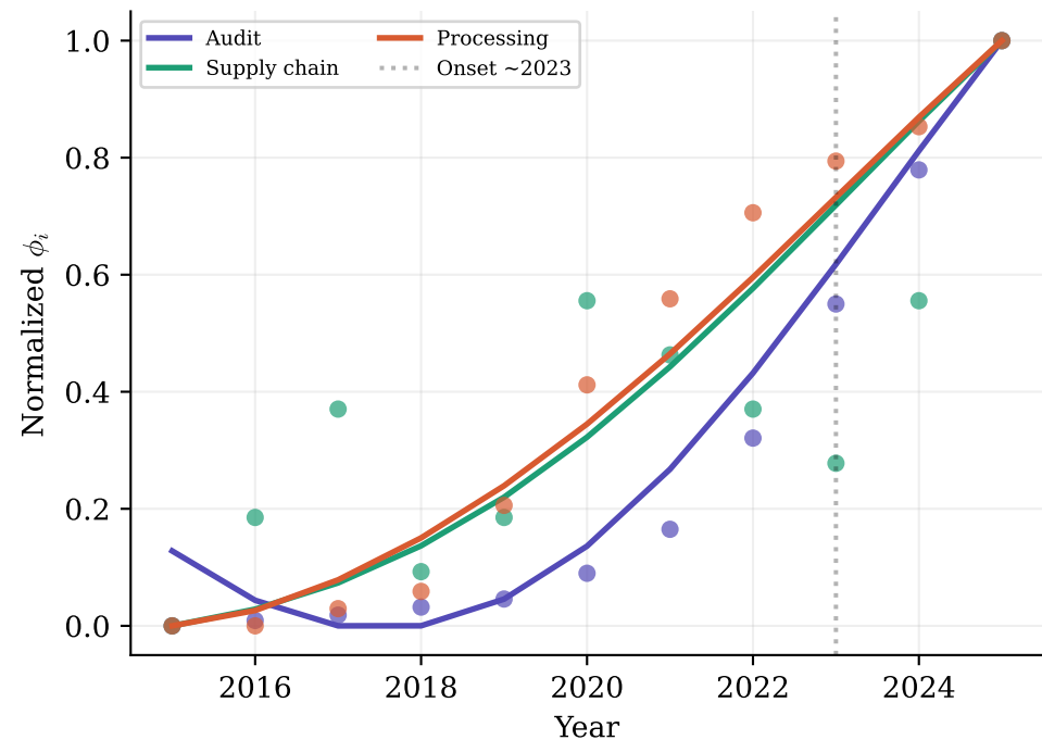
(a) Model fit vs. OpenAlex data
