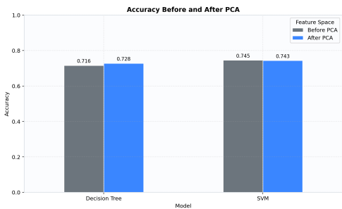
Figure 9A. Accuracy Before and After PCA
