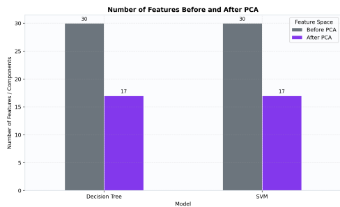
Figure 9B. Feature Count Before and After PCA
