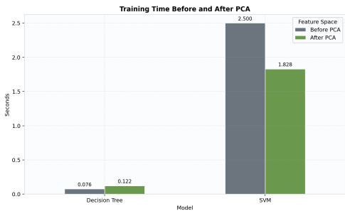
Figure 9C. Training Time Before and After PCA
