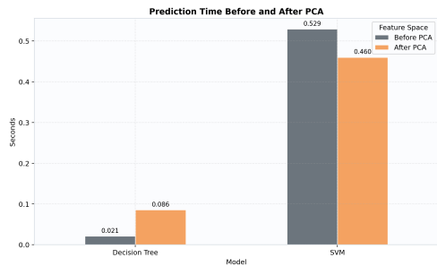
Figure 9D. Prediction Time Before and After PCA
