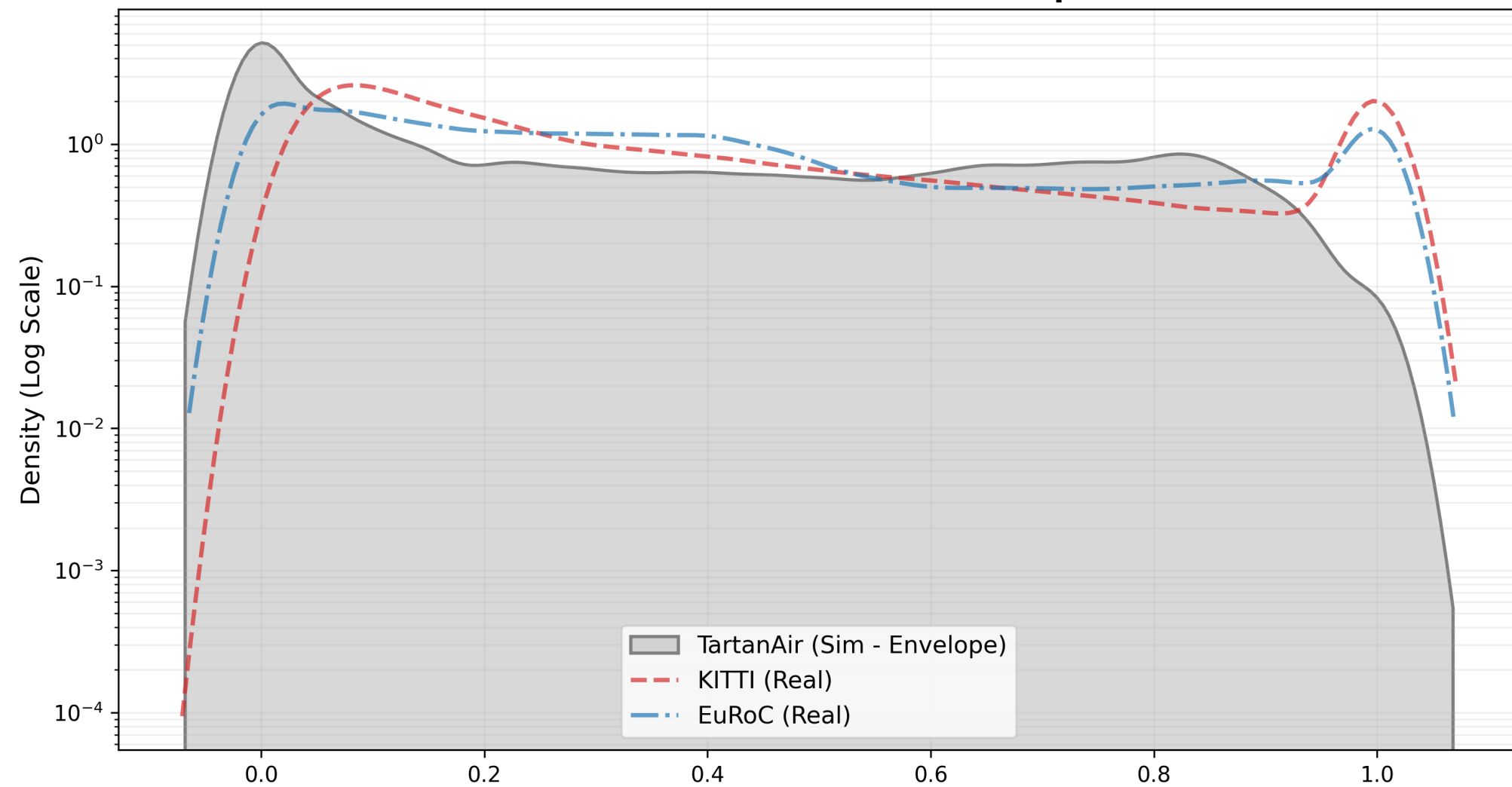
(a) Activation Value
