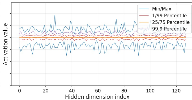
(b-2) SmoothQuant
