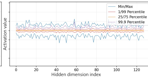
(d-2) Ours
