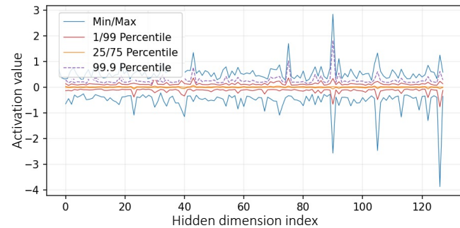
(a-2) Baseline
