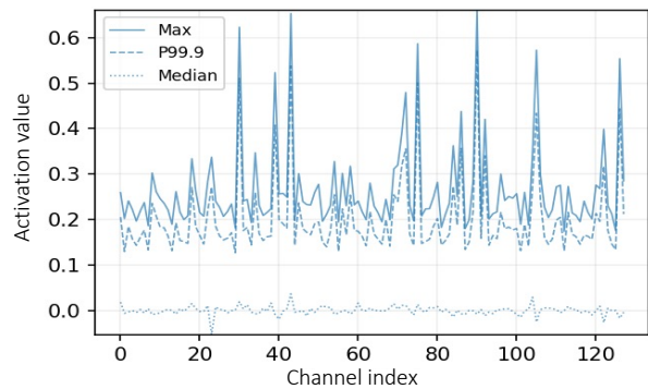
(a-1) Baseline
