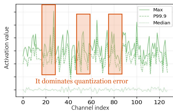
(b-1) SmoothQuant
