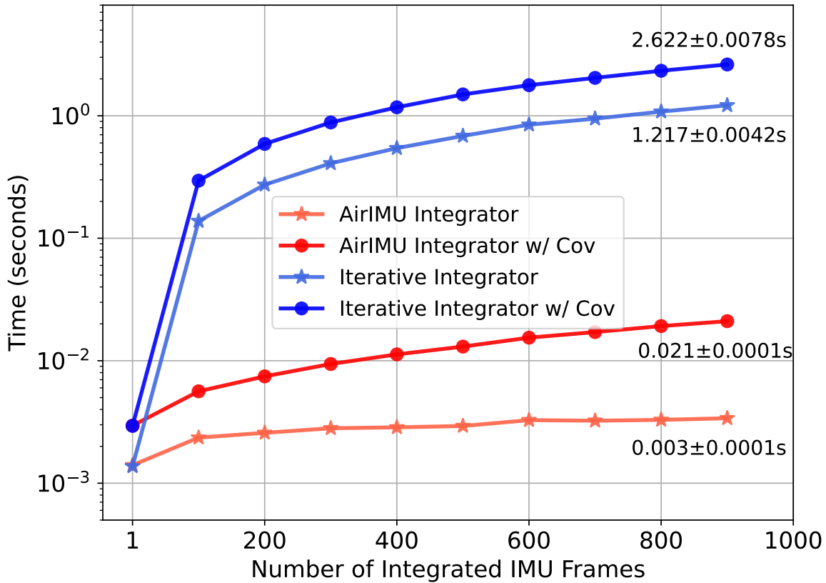
Figure 5.7: Time analysis of the AirIMU integrator compared to iterative methods. We integrate IMU input with different lengths (from 1 frame to 1000 frames) and display the time consumption on a log scale. The AirIMU integrator demonstrates a hundredfold improvement in efficiency.
