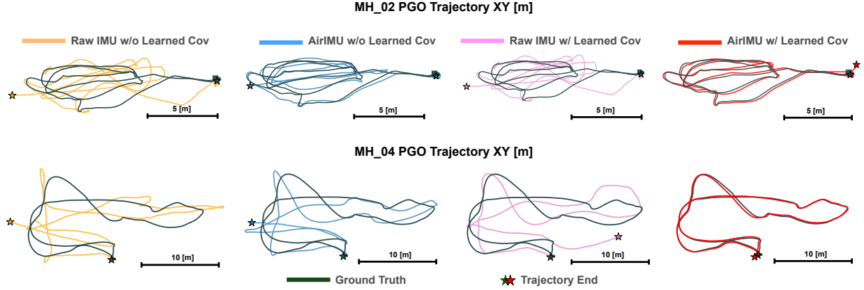
Figure 5.8: PGO results visualization showing the effectiveness of learned uncertainty in GPS-IMU fusion. The learned covariance from AirIMU enables more accurate and robust optimization compared to fixed uncertainty models.
