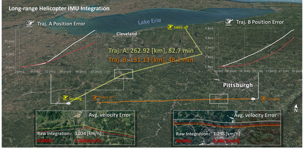
Figure 5.9: Near-earth helicopter navigation trajectory visualization over 262 km using navigation-grade IMUs. AirIMU enables precise long-term navigation in GPS-denied environments.
