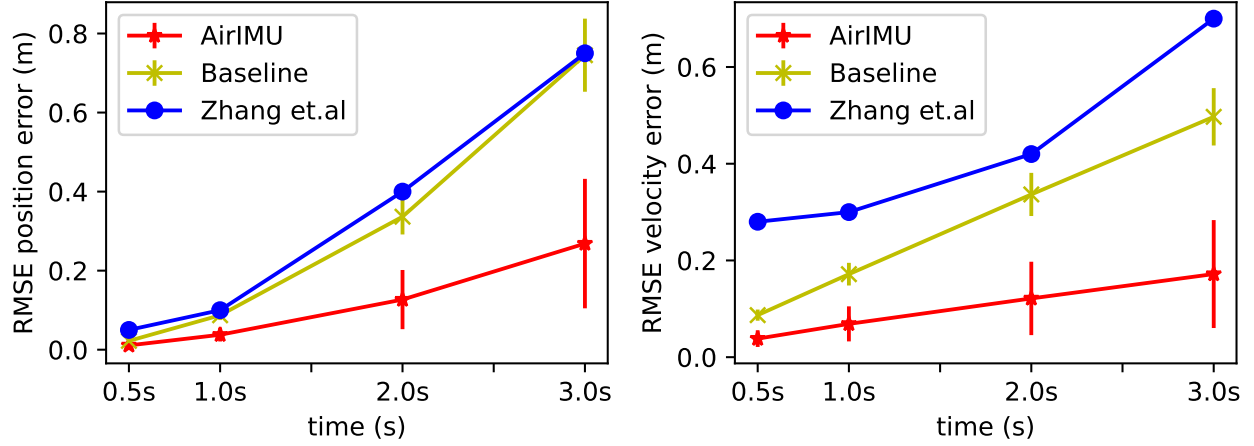
Figure 5.6: Integration results comparison showing AirIMU performance across different integration periods and datasets. AirIMU consistently outperforms baseline methods across various IMU grades and integration durations.
