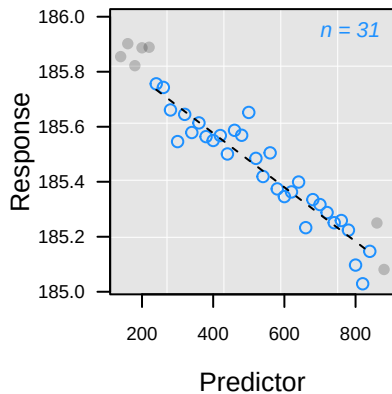
-- L_{pc} Rank 1: y = 185.97 - 0.0010 \cdot x
