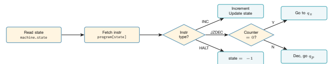
Fig. 3 — One reduce() iteration: read state, fetch, branch, update.
