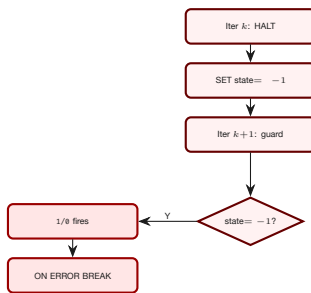
Fig. 2 — Termination via 1/0 + ON ERROR BREAK .
